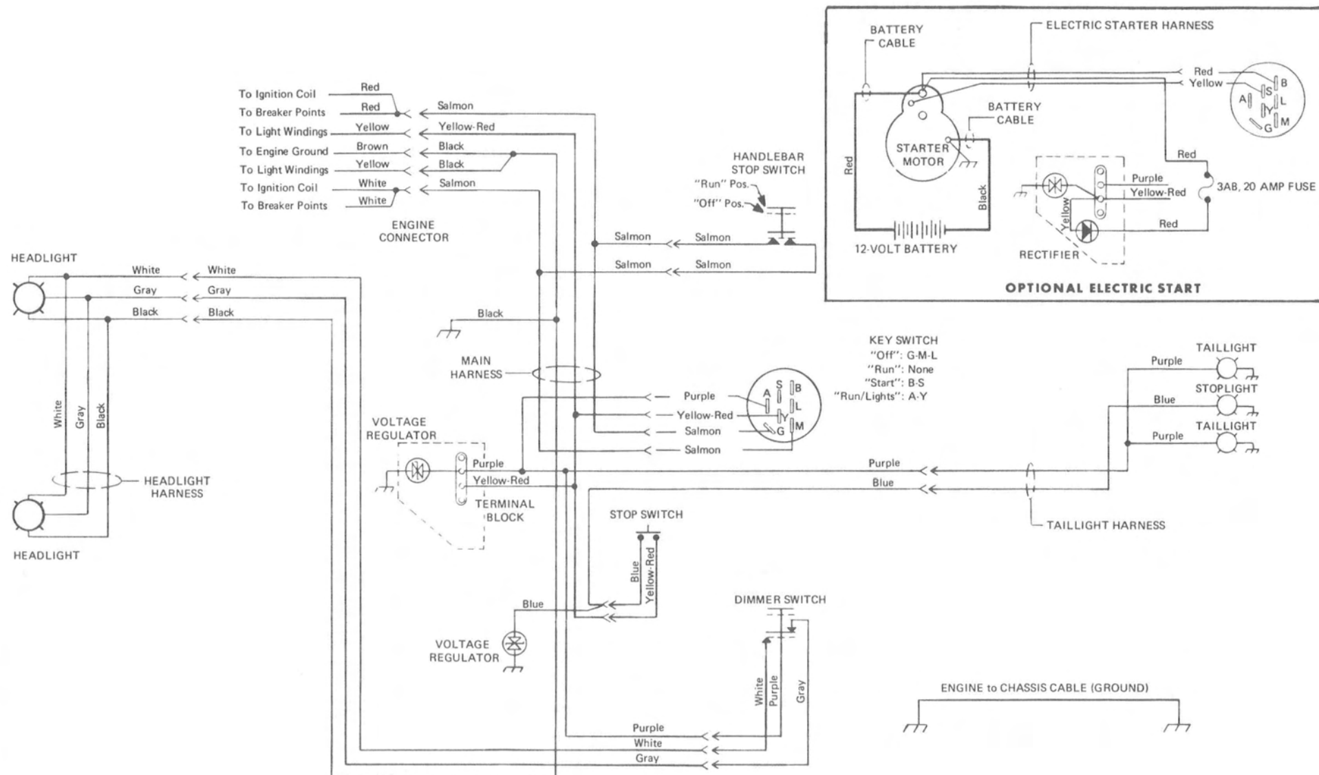
Figure 11. Model 440 MAX (CHASSIS Serial No. 3447382 and Below) Wiring Diagram
