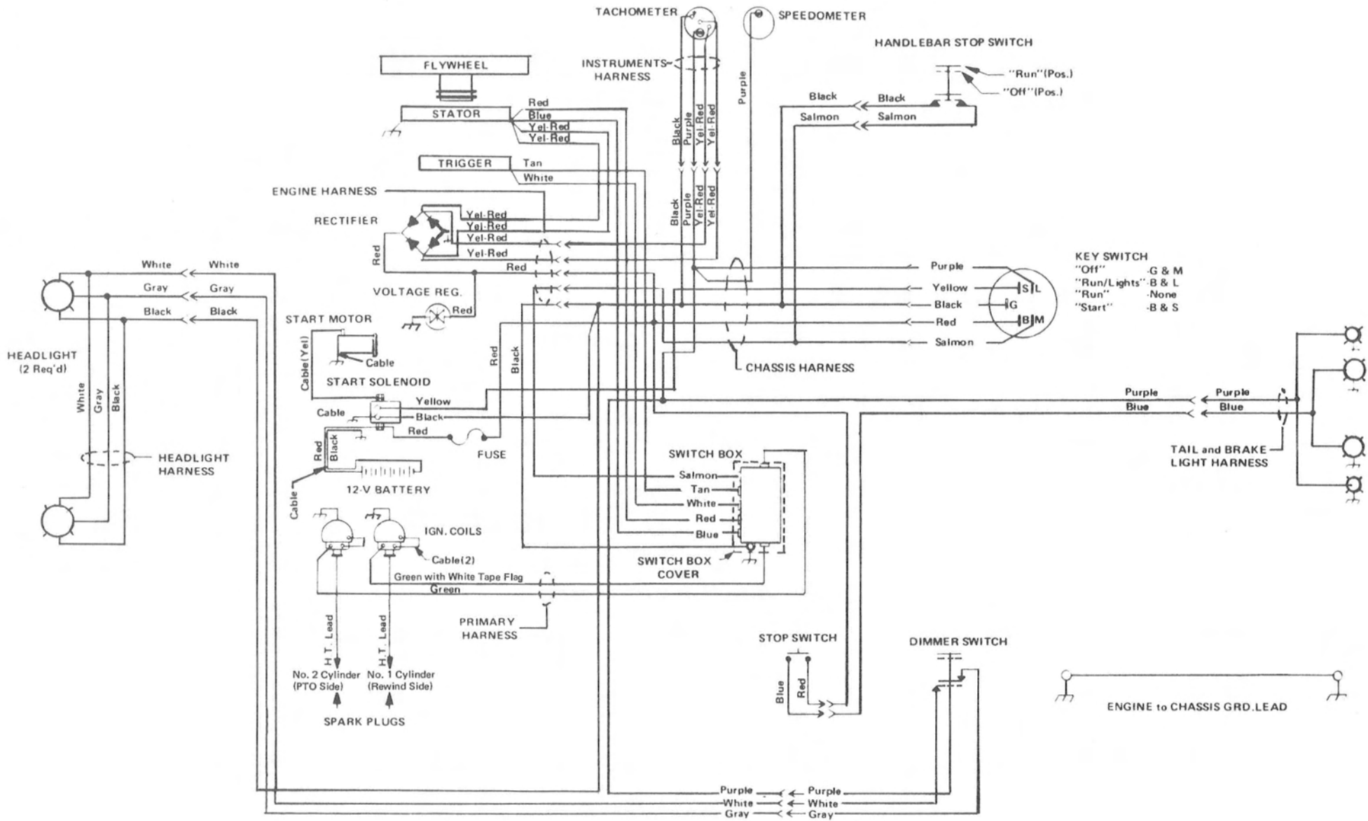
Figure 12. Model Mark I and Mark II (CHASSIS Serial No. 3591478 and Below) Wiring Diagram
