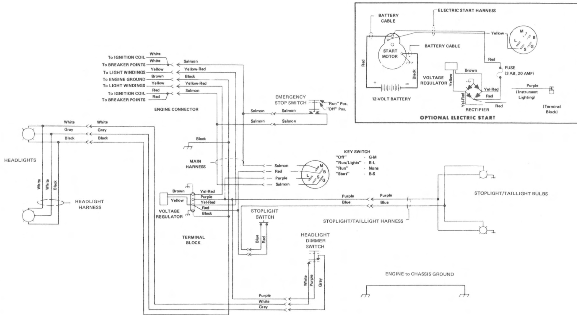
Figure 13. Models 440 MAX, 440 M/X and 440 S/R with CHASSIS Serial No. 3709838 thru 4064696 Wiring Diagram
