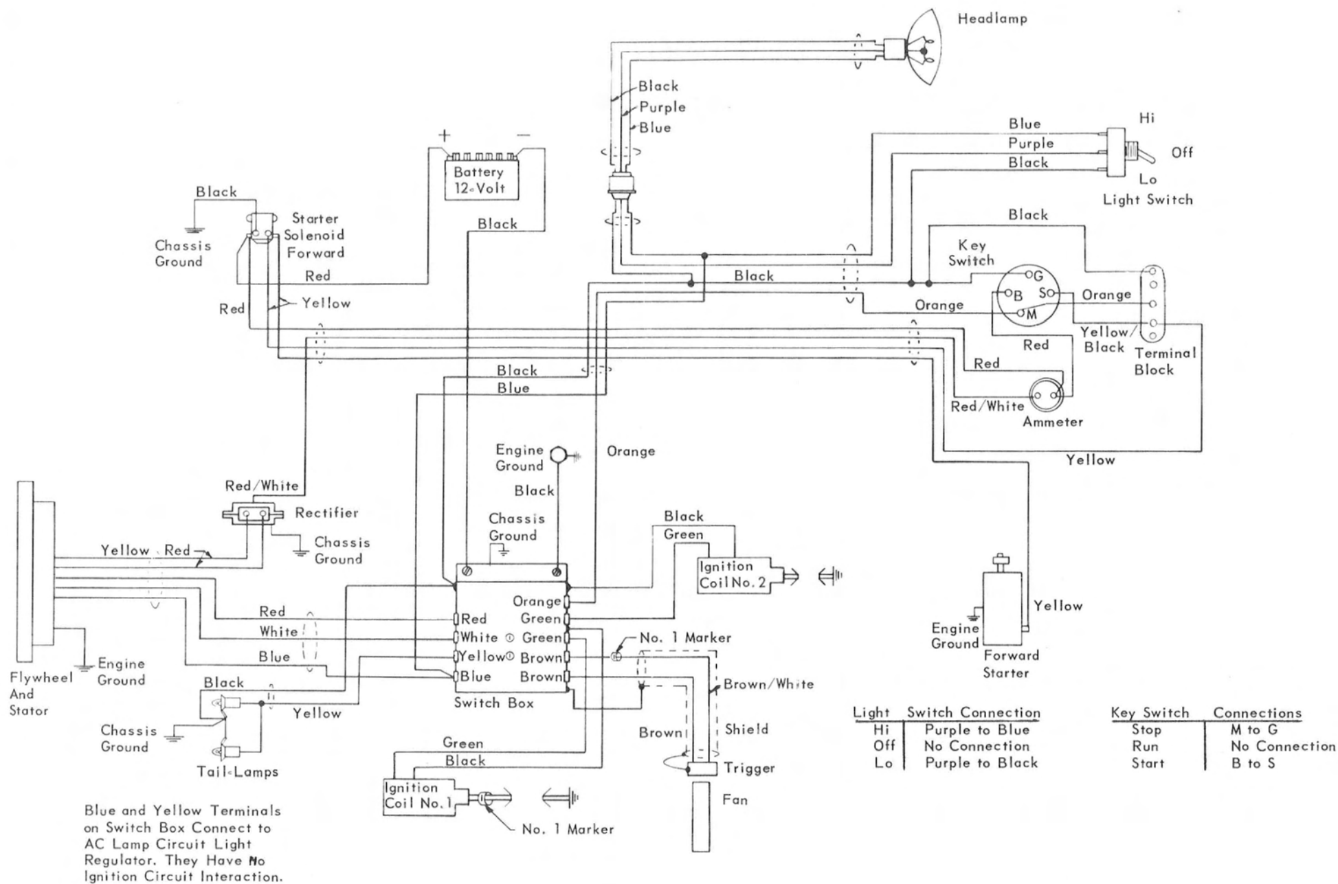
Figure 2. Model 220E Wiring Diagram
