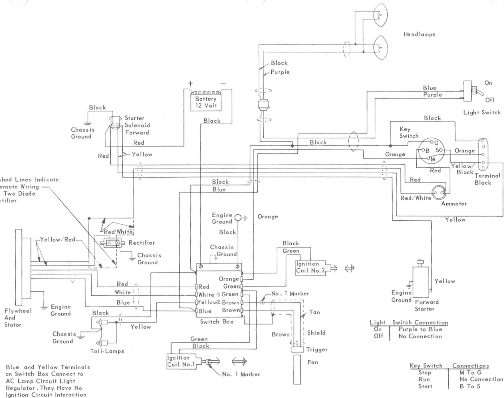
Figure 5. Model 250E Wiring Diagram
