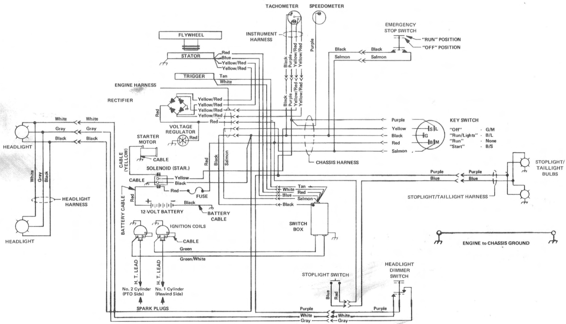
Figure 14. Model Mark II (CHASSIS Serial No. 3787640 and Above) Wiring Diagram
