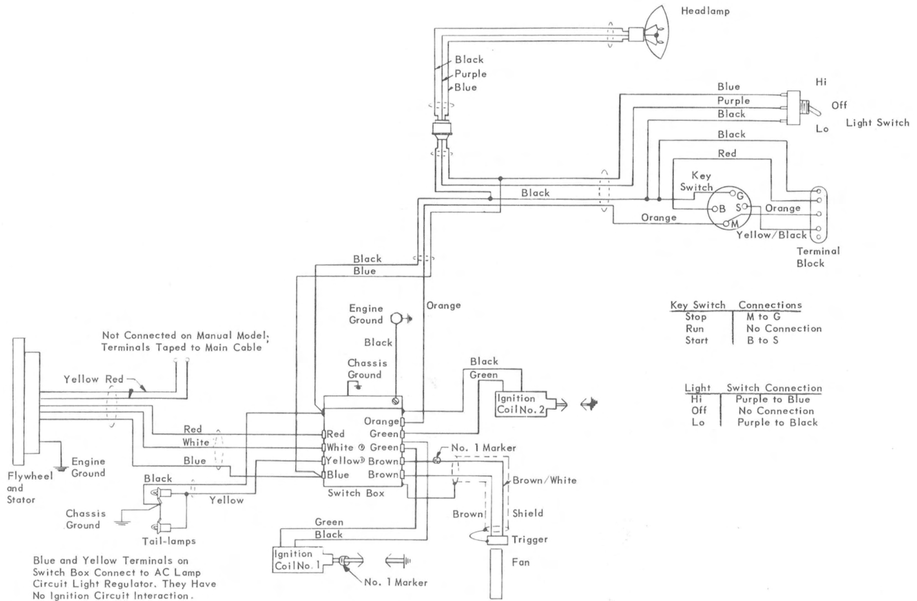
Figure 1. Model 220M Wiring Diagram
